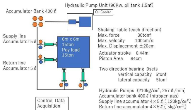
YTIT X, Y Two Horizontal Direction Shaking Table Hydraulic Power Supply Initial Setting
