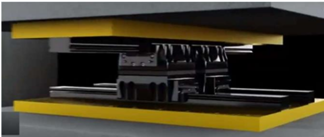
Fig.10 Two Horizontal Direction Bearing of THK Company
